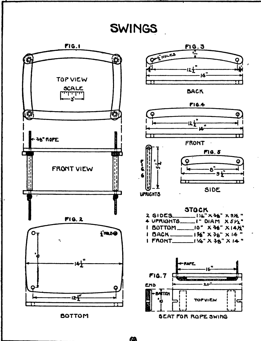
Fig. 7 is a seat for the ordinary rope swing. Batten pieces should be fastened underneath across each end. The sharp corners of the wood should be rounded off wherever the rope touches it, to prevent cutting the rope.
